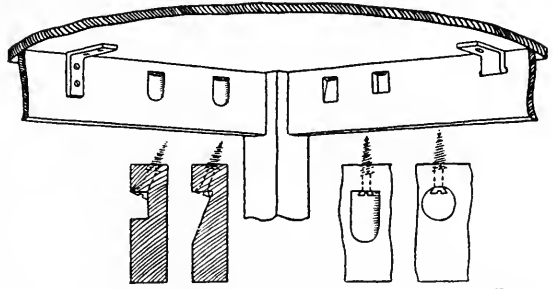
FIG. 424. FASTENINGS FOR TABLE TOPS.
